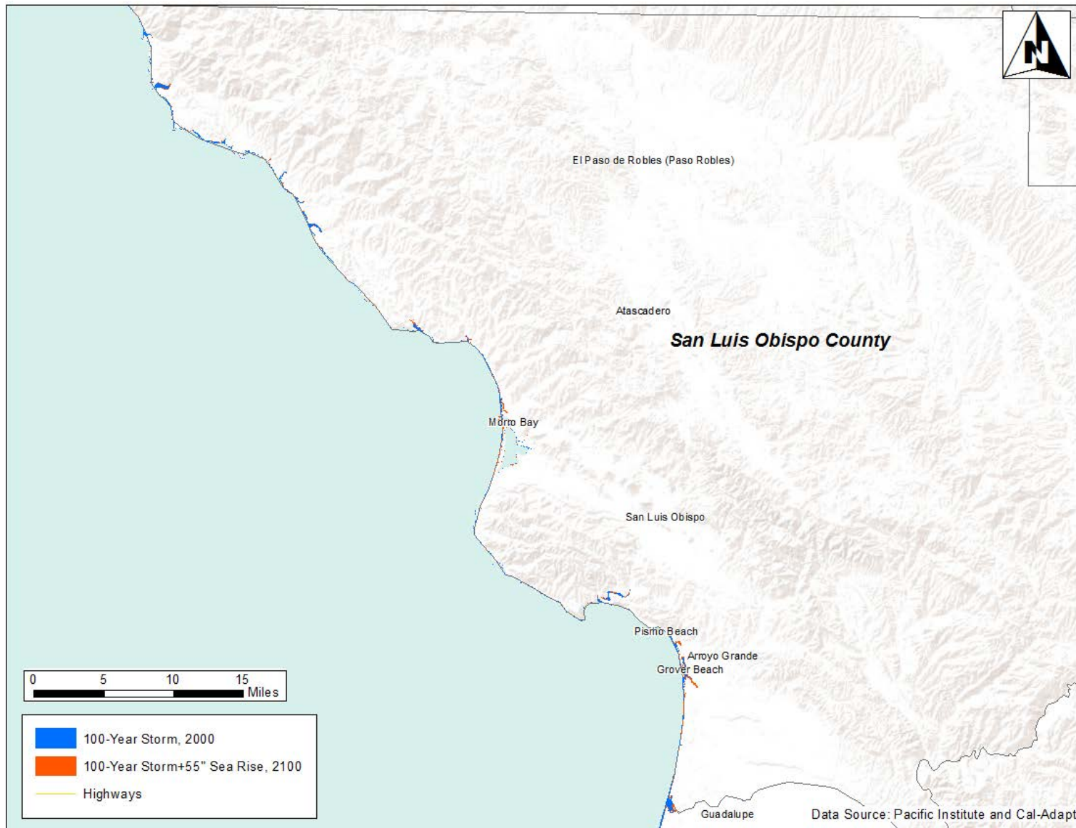
Figure 5. Baseline inundation areas for a 100-year flood (2000) and modeled scenario with additional 55 inches of sea level rise (2100), San Luis Obispo County 6 Note: Current projections are 66 inches above sea level. 7
