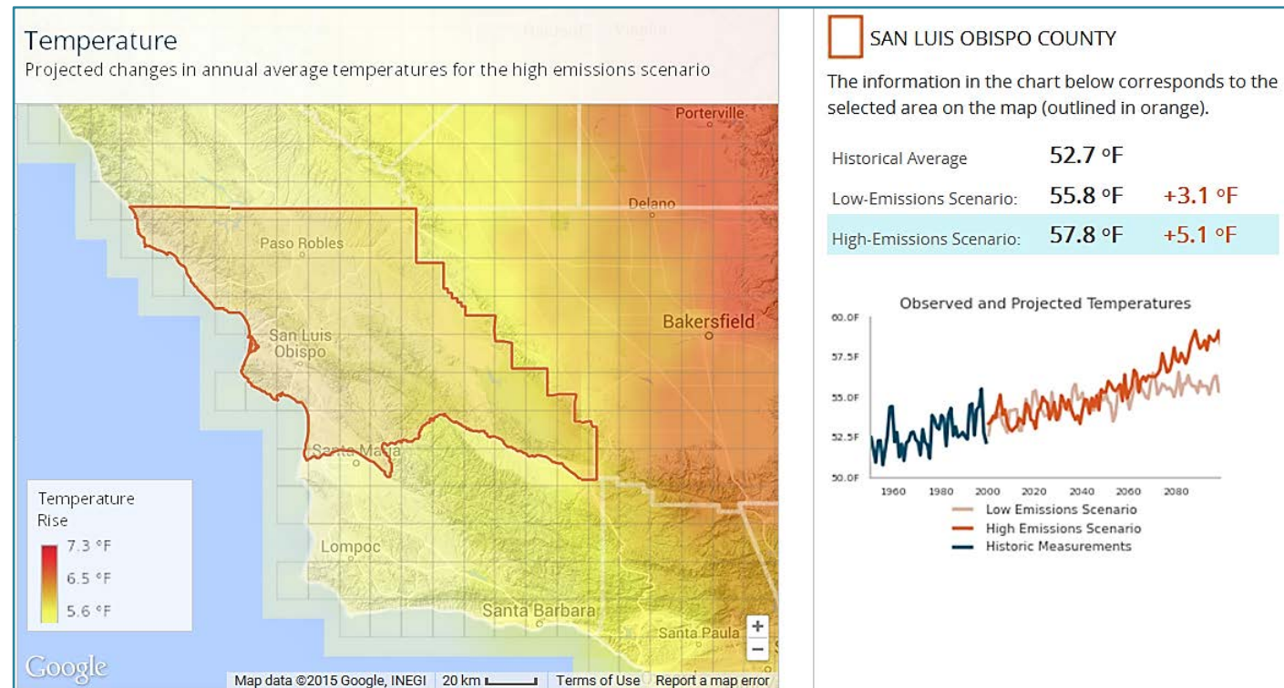
Figure 2. Projected changes in annual average temperature in future carbon emissions scenarios, San Luis Obispo County, 2099 6
