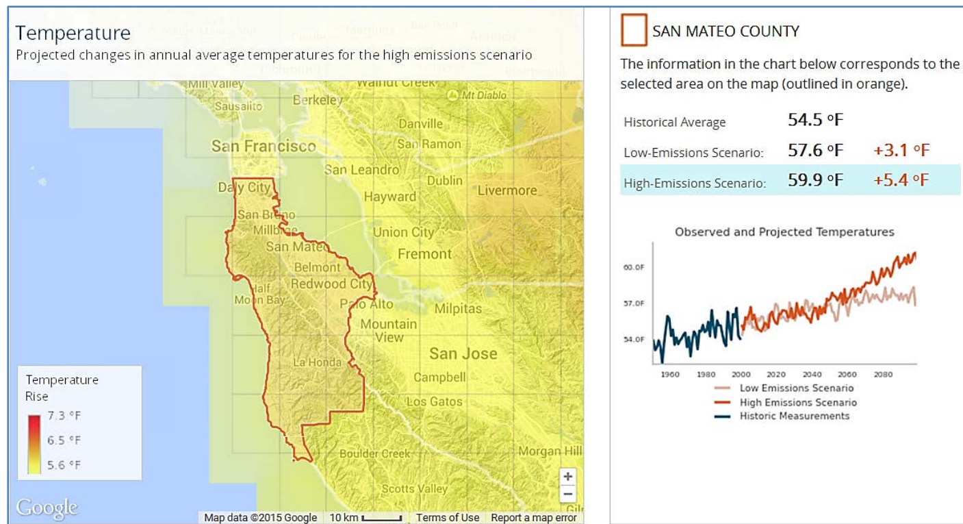
Figure 2. Projected changes in annual average temperature in future carbon emissions scenarios, San Mateo County, 2099 6
