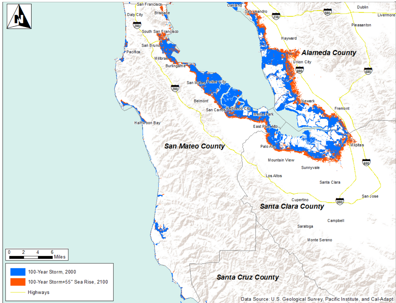
Figure 5. Baseline inundation areas for a 100-year flood (2000) and modeled scenario with additional 55 inches of sea level rise (2100), San Mateo County 6 Note: Current SLR projections are 66 inches above sea level. 7
