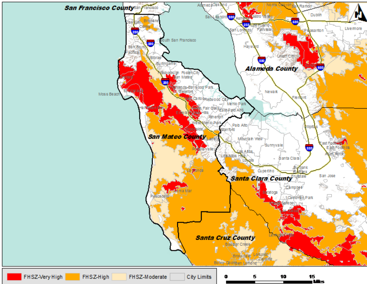
Figure 3. Current Fire Hazard Severity Zones (FHSZ), San Mateo County, 2007 9
