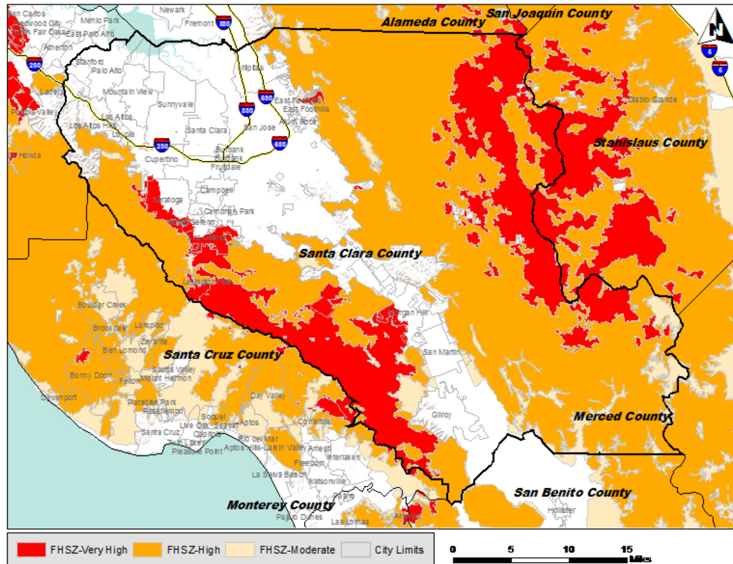
Figure 3. Current Fire Hazard Severity Zones (FHSZ), Santa Clara County, 2007 9
