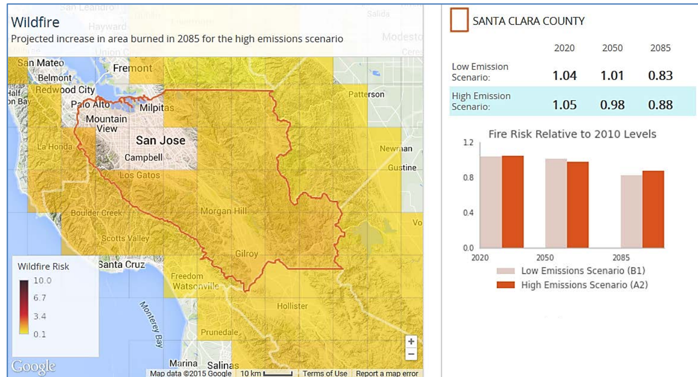
Figure 4. Relative increase in wildfire acreage in future carbon emission scenarios, Santa Clara County 6
