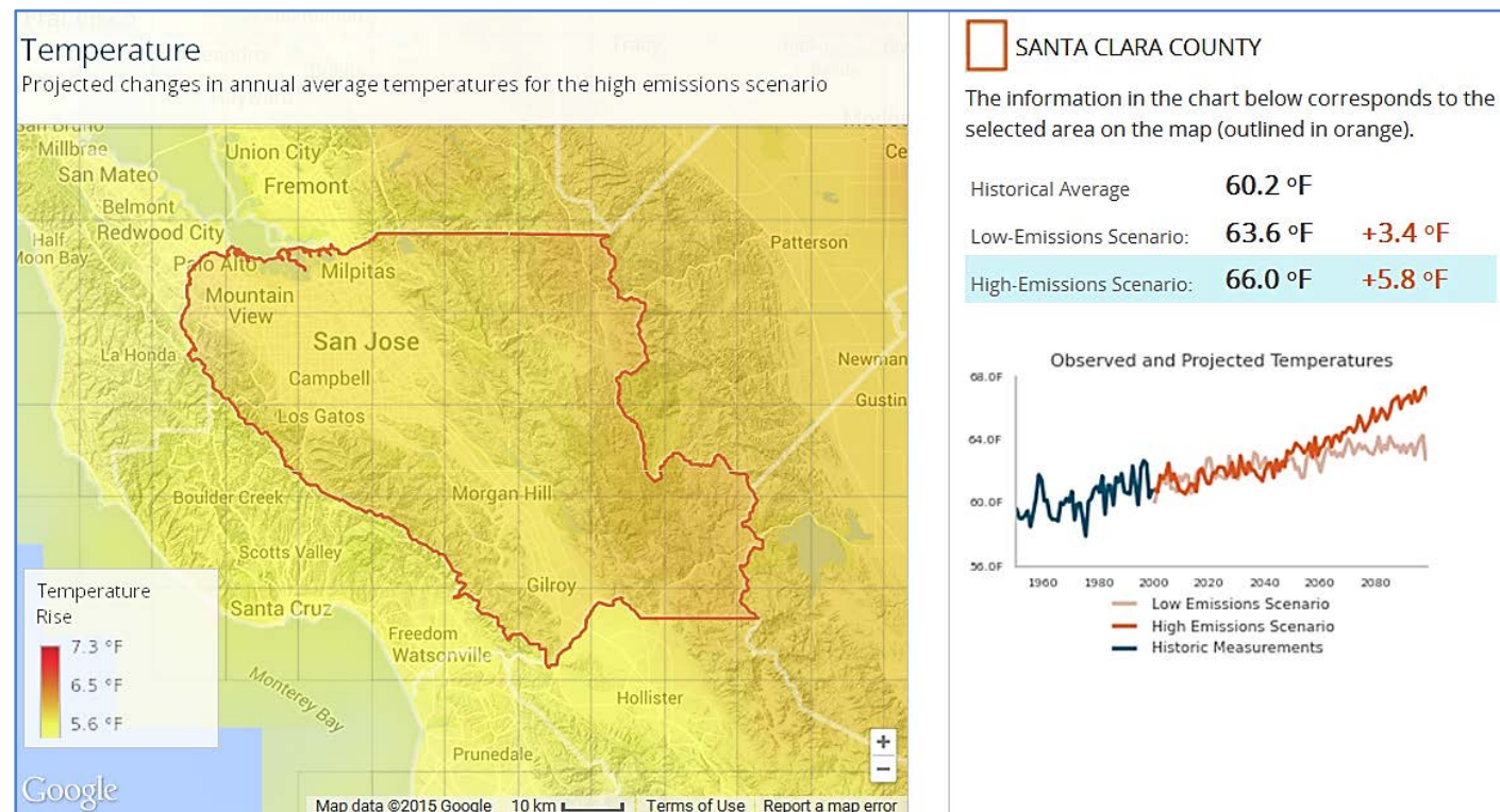
Figure 2. Projected changes in annual average temperature in future carbon emissions scenarios, Santa Clara County, 2099 6
