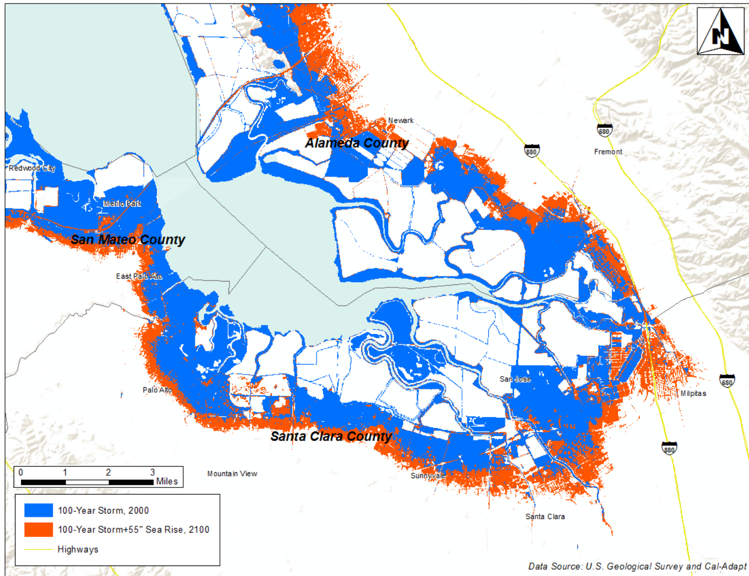
Figure 5. Baseline inundation areas for a 100-year flood (2000) and modeled scenario with additional 55 inches of sea level rise (2100), Santa Clara County 6 Note: Current projections are 66 inches above sea level. 7
